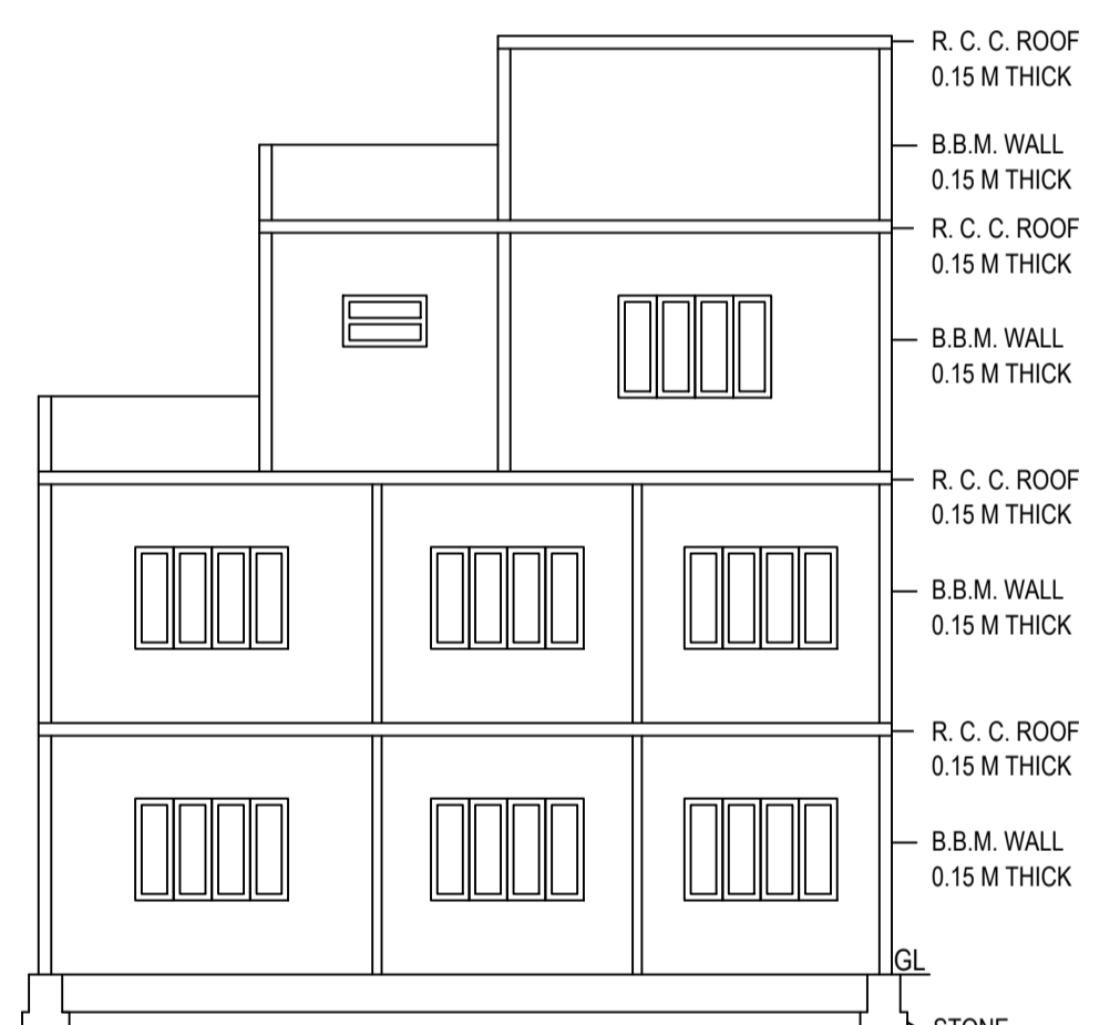
SECTION
