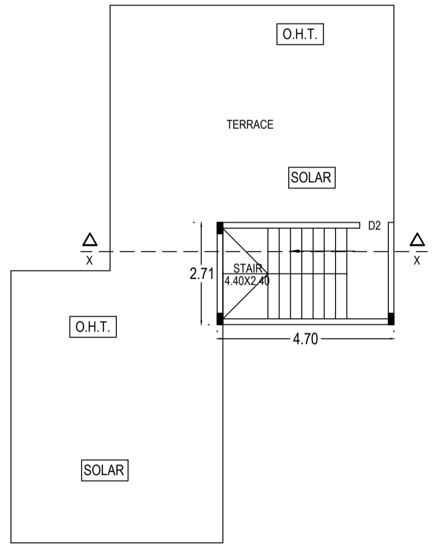
TERRACE FLOOR
