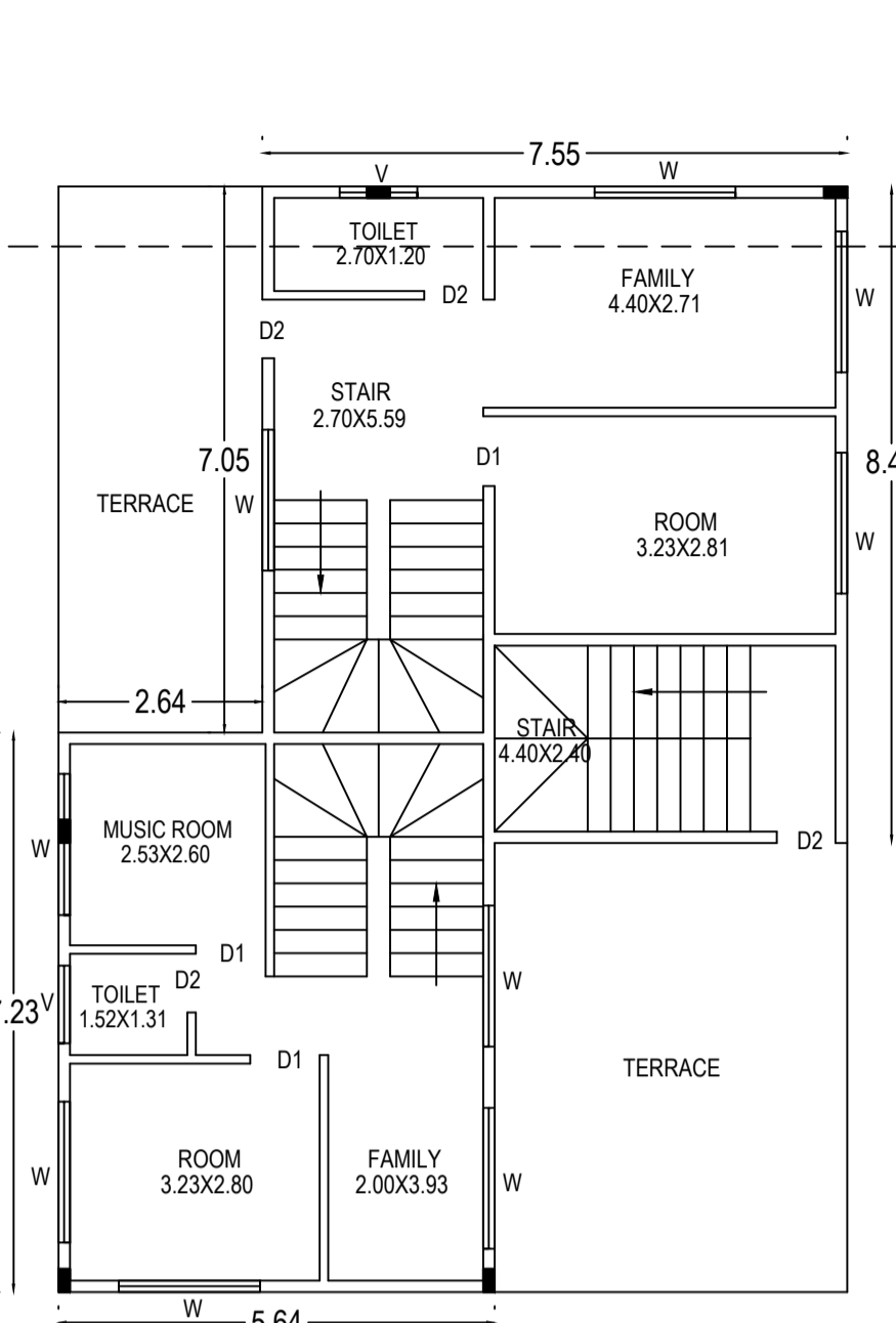
SECOND FLOOR
