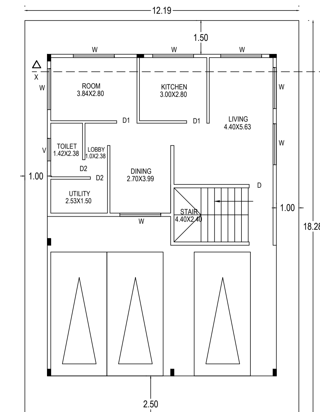
GROUND FLOOR
