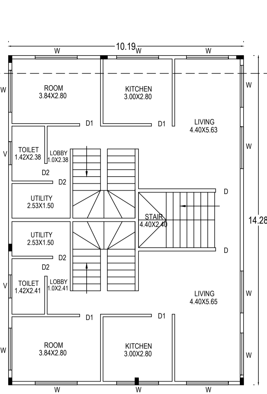
FIRST FLOOR
